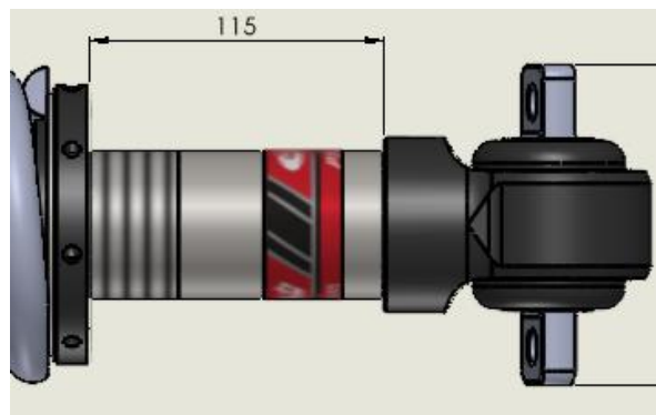
Set preload to 115mm/4.5" for level with OE rear for 2.7L EcoBoost.
