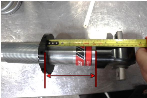
11. Verify pre-load of the coilover by measuring from the bottom of the lower spring perch to the top of the lower shock mount. Out of the box this setting should be 107mm which will provide a ride height level with the OE rear suspension. Exceeding 3" of lift will result in poor ride quality.
